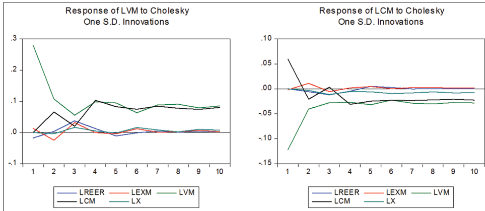
Figure 1: Response to the unit shocks on LVM and LCM
